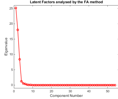
Fig. 5. Latent Factors achieved by using FA
